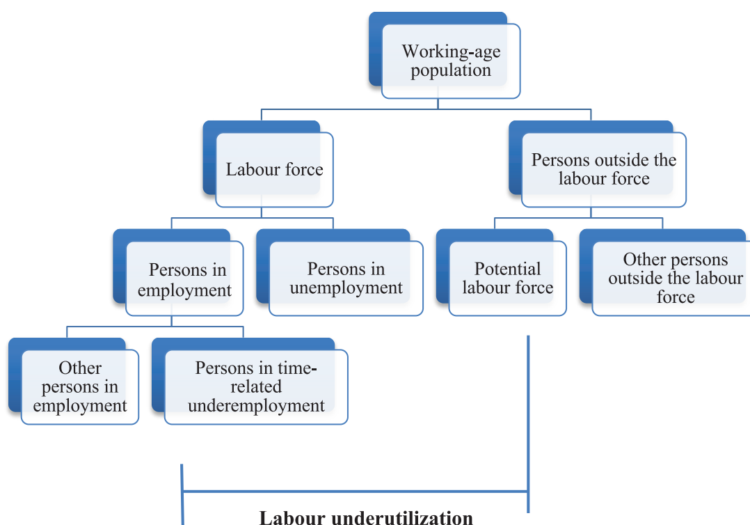
Figure 7.1 Measurement framework
